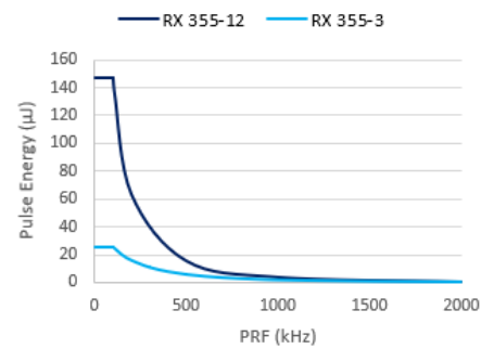
Typical Single Pulse Energy Output
