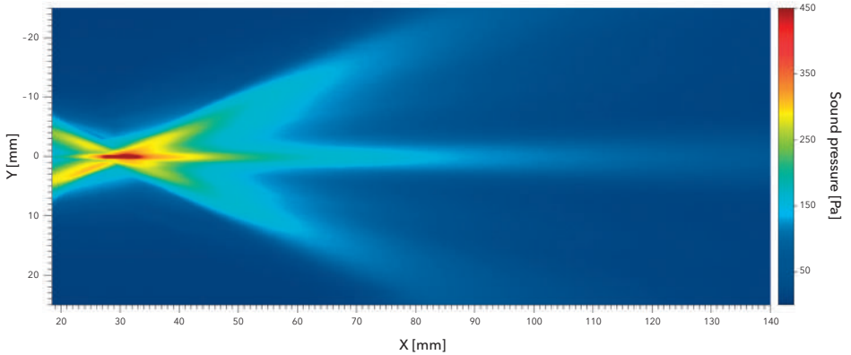
Acoustic field of a thermoacoustic emitter measured with an Optical Microphone
