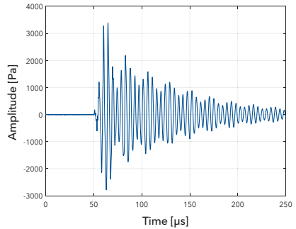
Impulse response of a piezoelectric emitter
